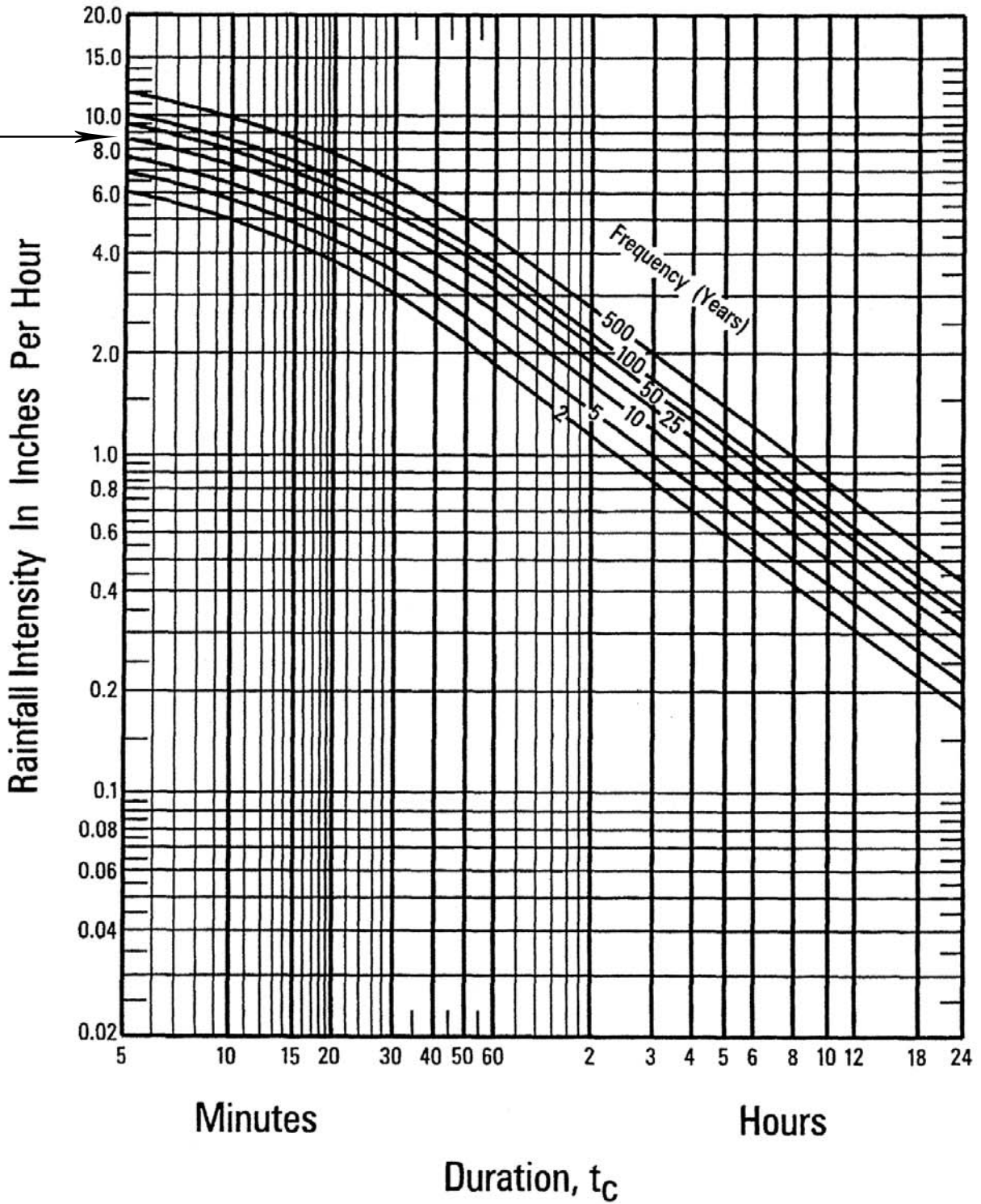
RAINFALL INTENSITY - DURATION - FREQUENCY CURVES City of Starkville, MS
